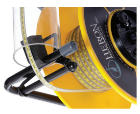
Figure 3 Hanger to support the meter at the well head. Tape Guide to protect the tape from sharp edges.
