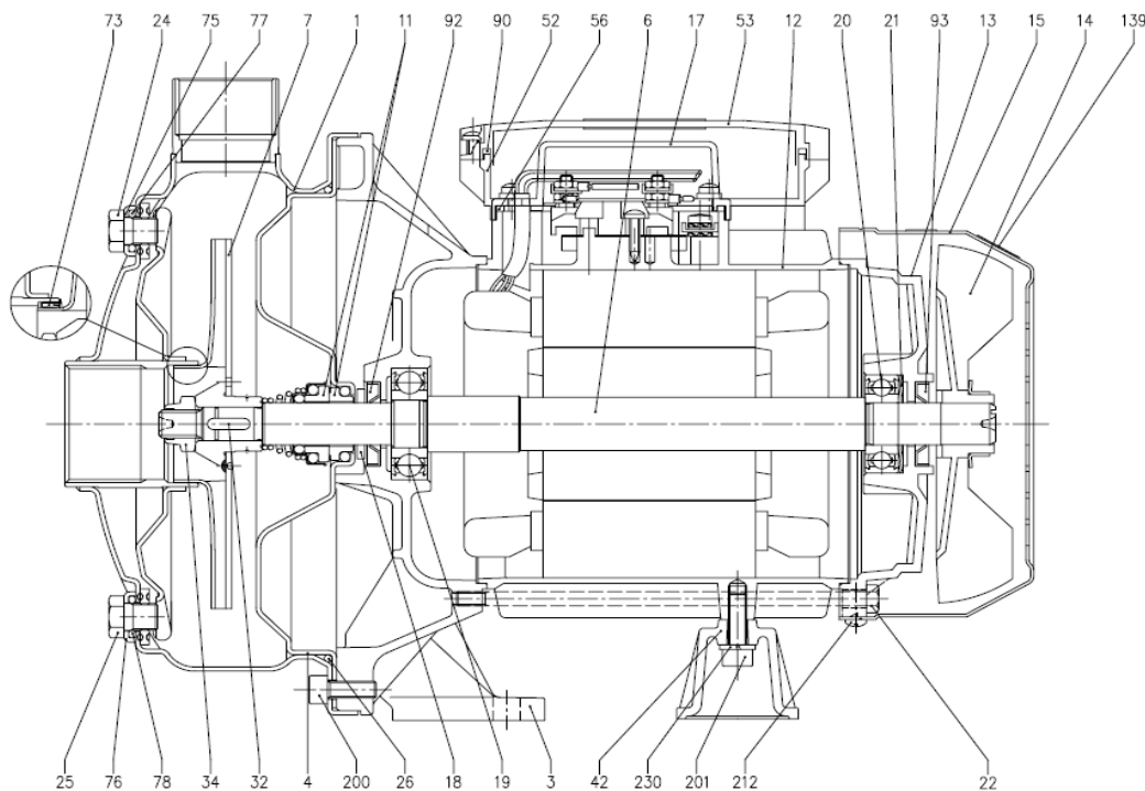
CDX/CDXM Parts
