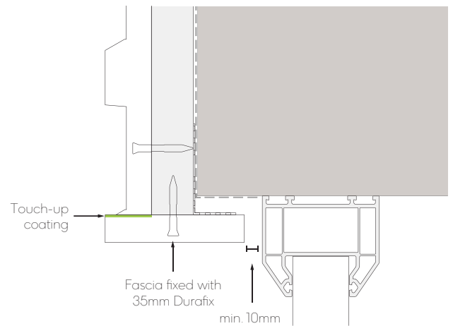
Fig. 15 - Window/door head with fascias
