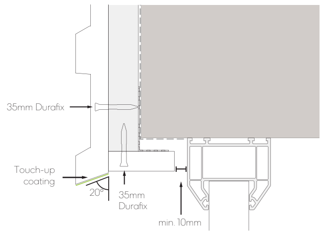
Fig. 14 - Window/door head with angled cut
