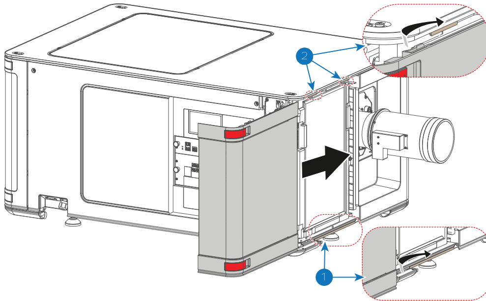
Image 21-4 Sliding in the front cover
