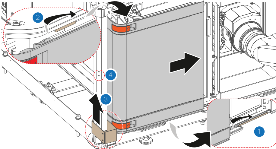
Image 22-8 Sliding in the front cover
