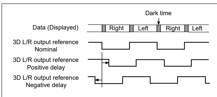
Image 8–88 Delay example for 3D L/R Output Reference
