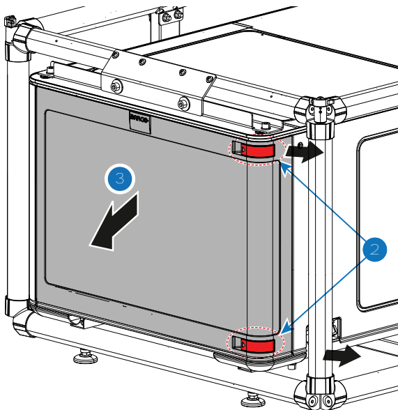
Image 22-4 Sliding the front cover towards the frame bar and removing it.
