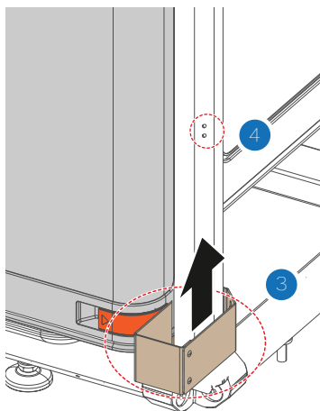
Image 22-6 Positioning the safety bracket
