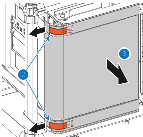
Image 22-2 Sliding the front cover towards the frame bar and removing it.
