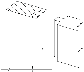
Stub Mortise & Tenon
