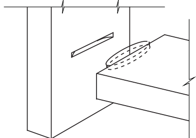
Biscuit Spline
