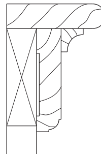
8 Chair Rail Combination (Cap, cove & rail) Running Trim
