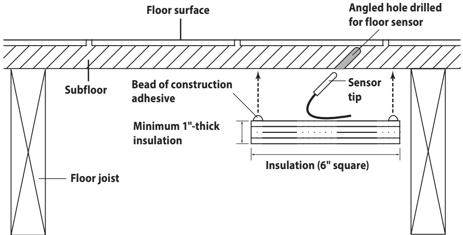
Diagram showing Method 1 for installing the floor sensor into the subfloor.
