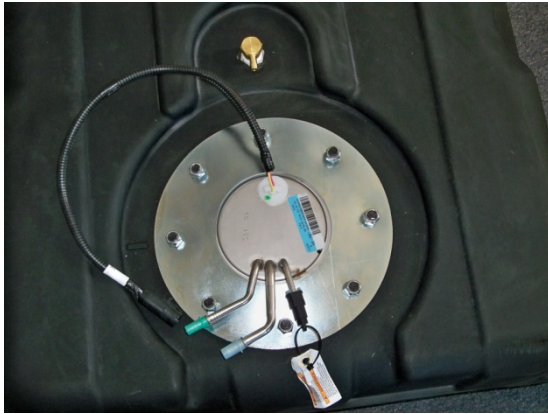
(Fig. 13) PS-191 Sending Unit Installed in TITAN tank.
