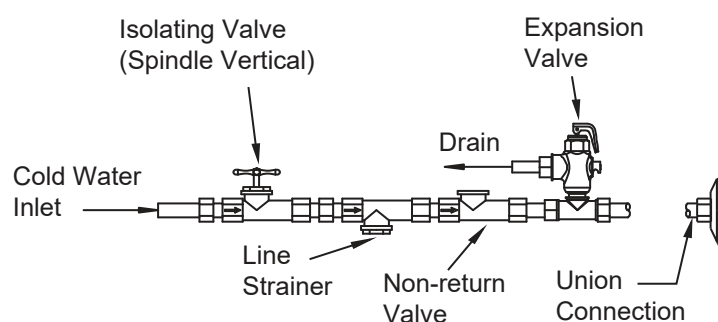
Figure 3. Inlet Connections
