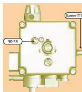
Figure 7. Adjusting the "NO P.R." Screw
