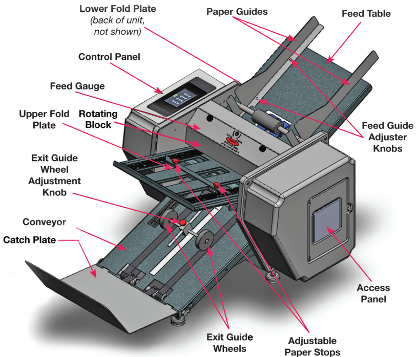
Figure 6: Machine Diagram
