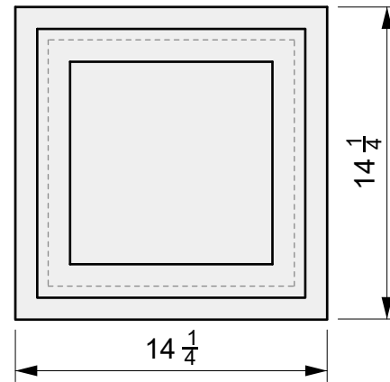
01 TOP VIEW
