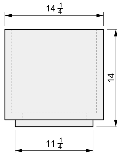
02 FRONT VIEW
