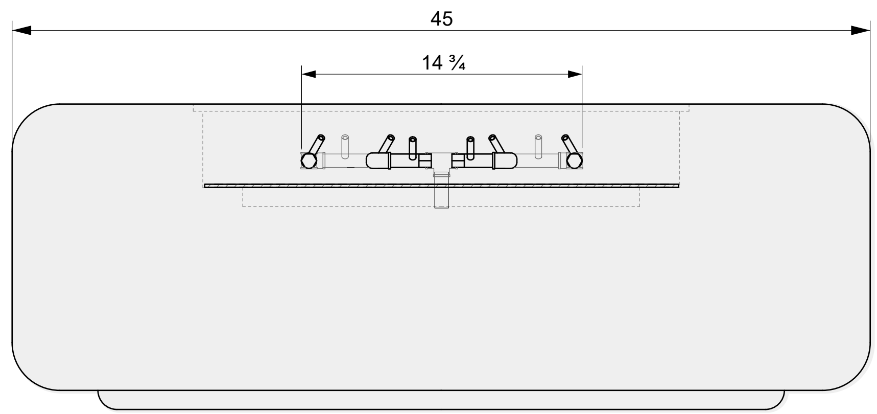
01 SIDE VIEW
