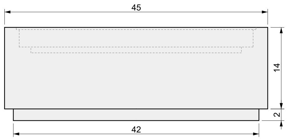
02 FRONT VIEW
