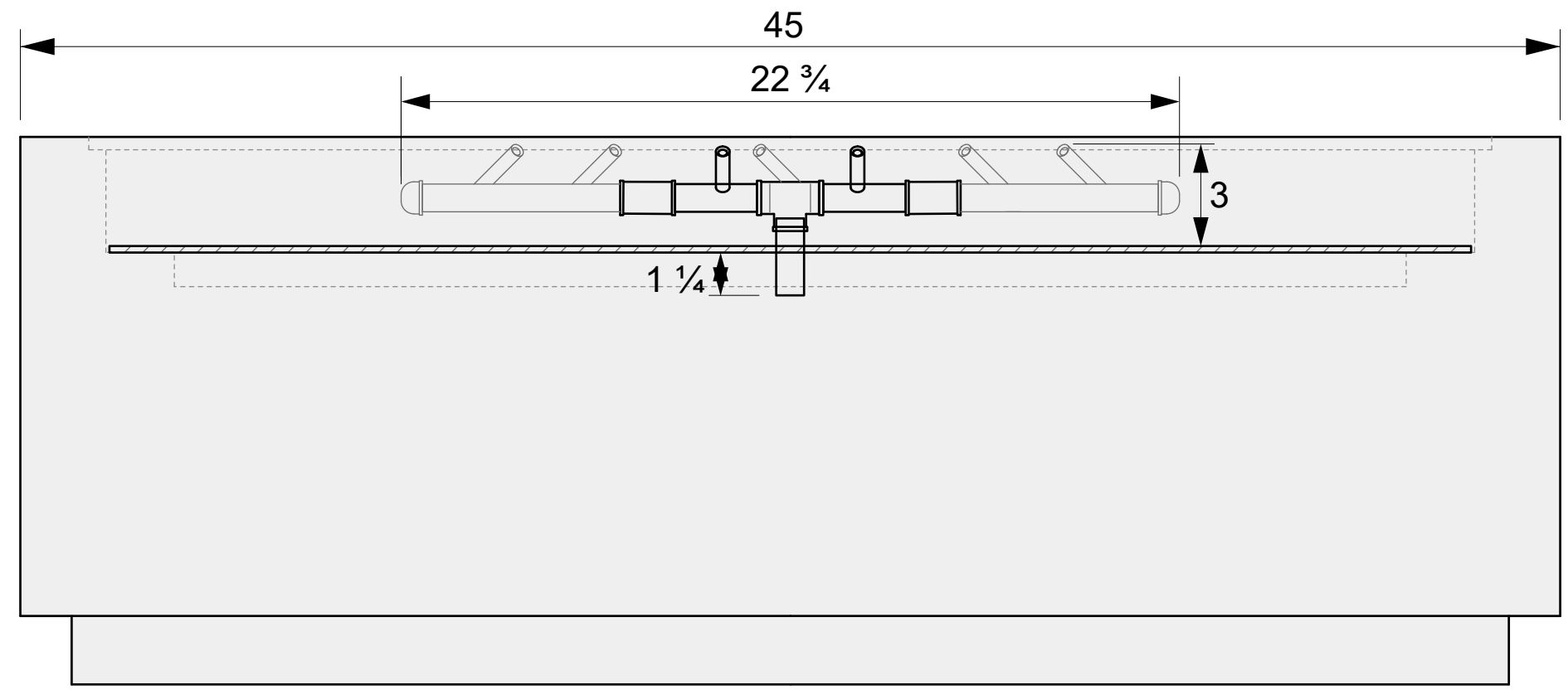
01 SIDE VIEW
