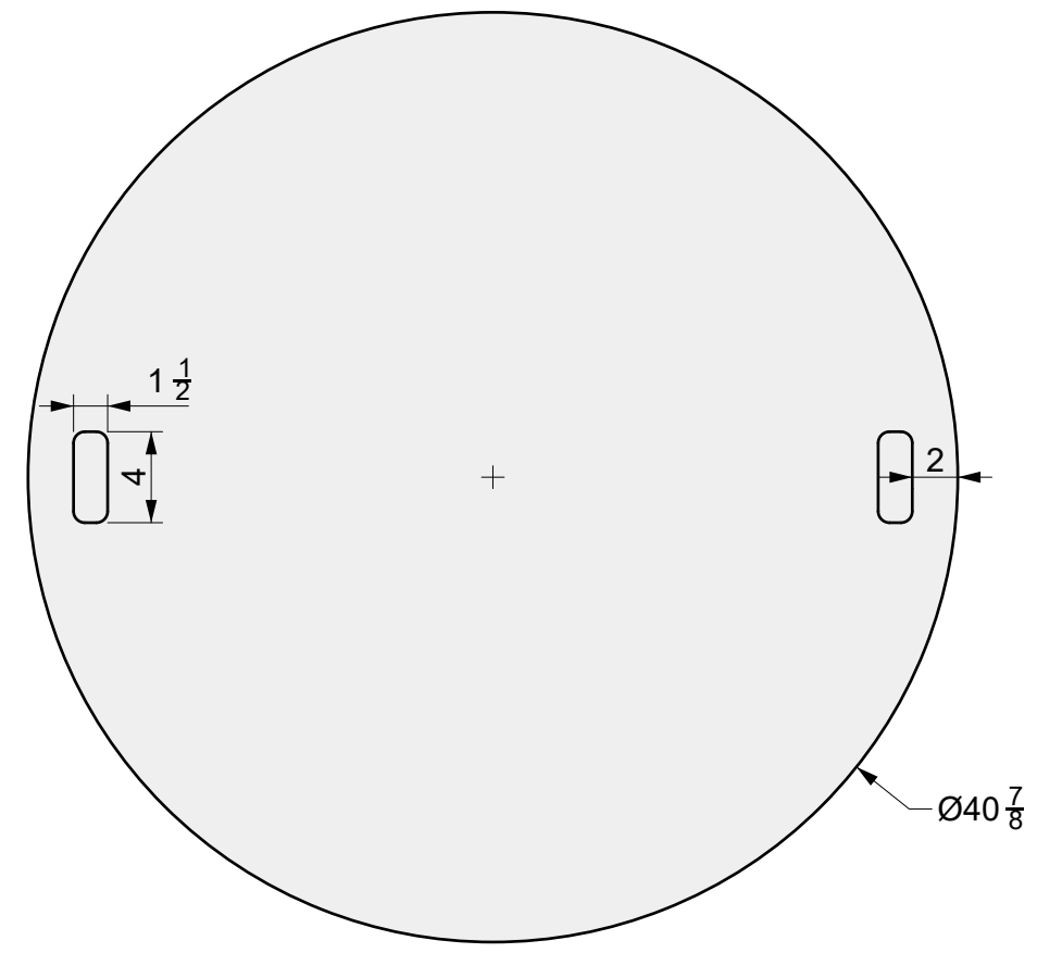
01 TOP VIEW
