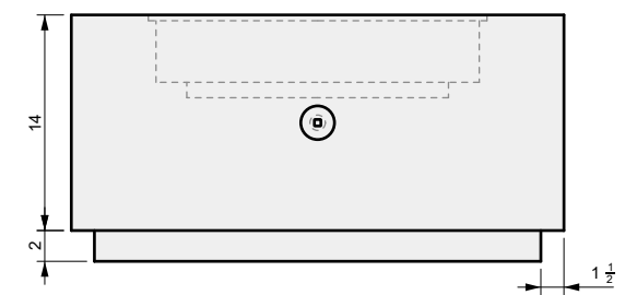
03 SIDE VIEW
