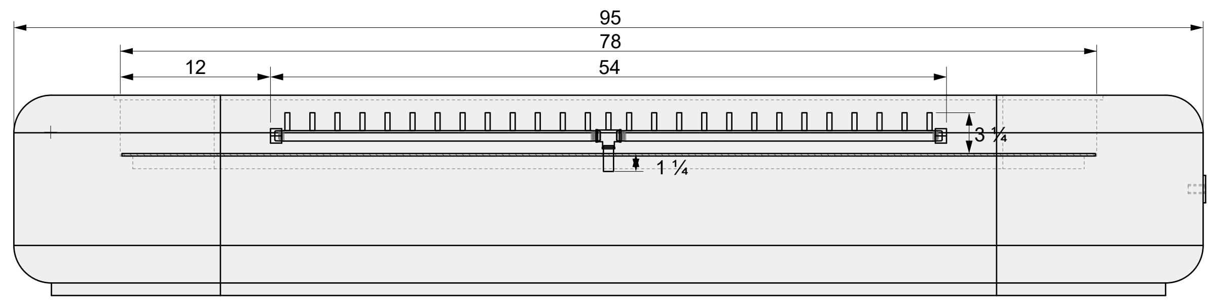
01 SIDE VIEW
