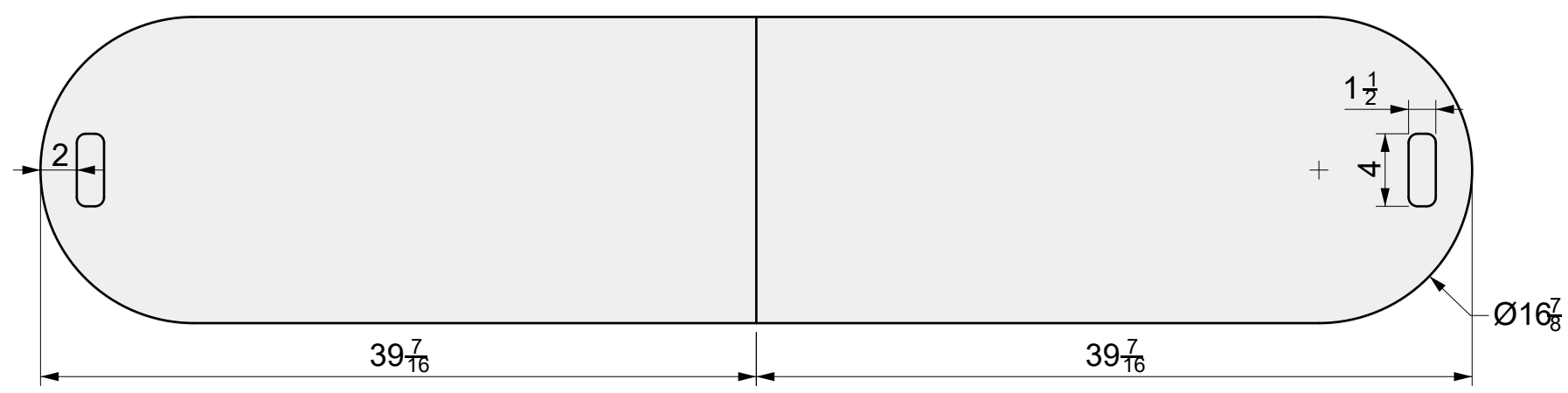
01 TOP VIEW
