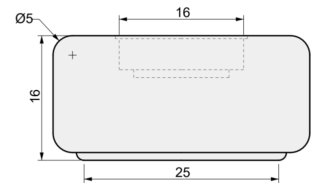
03 SIDE VIEW
