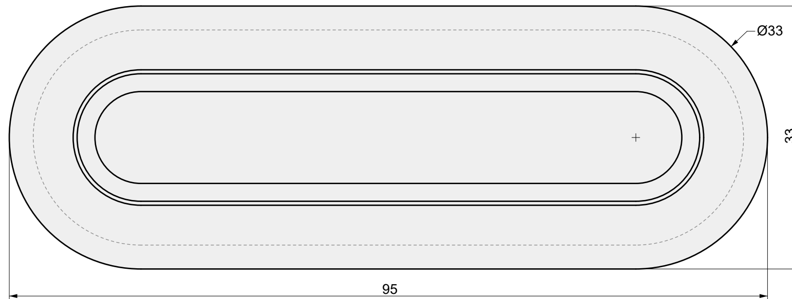
01 TOP VIEW
