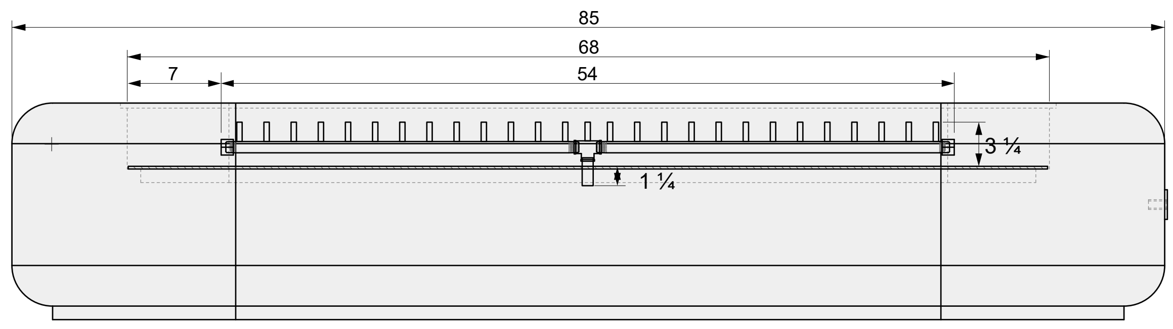
01 SIDE VIEW
