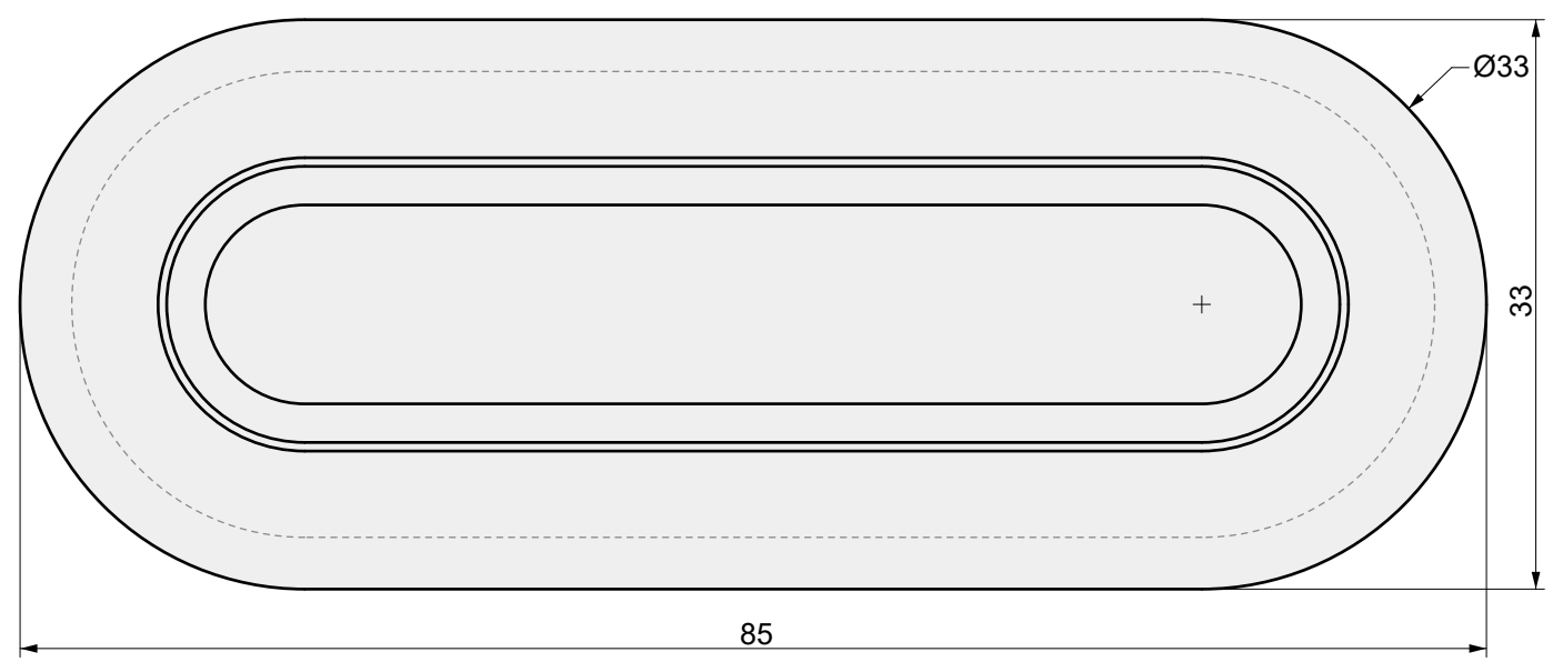
01 TOP VIEW
