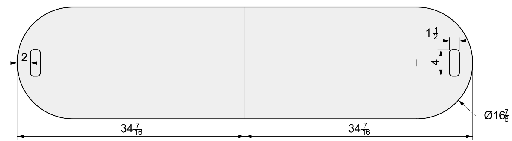
01 TOP VIEW
