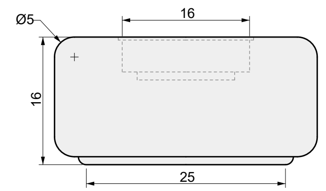
03 SIDE VIEW
