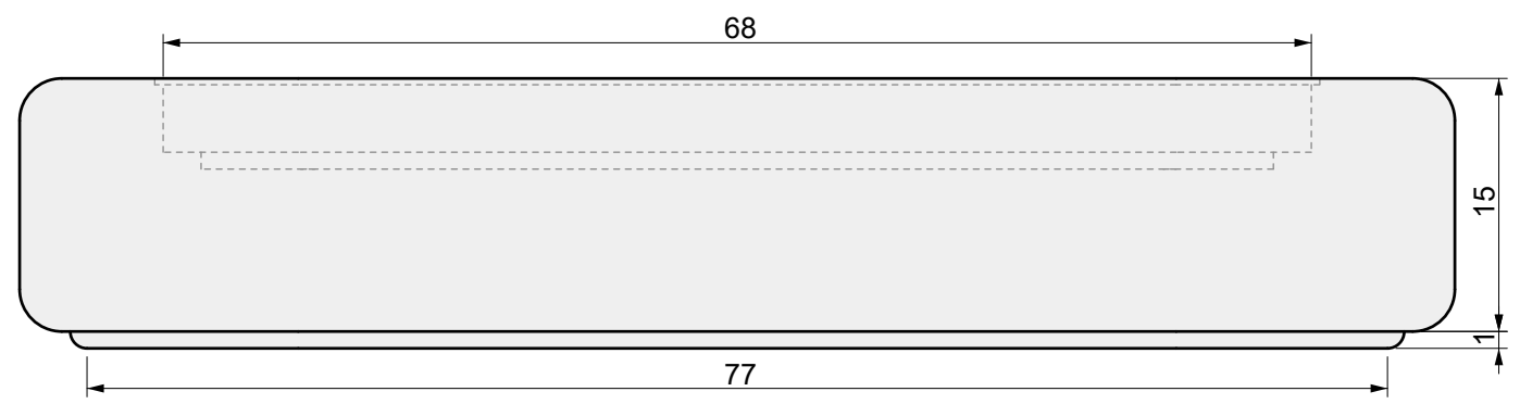
02 FRONT VIEW
