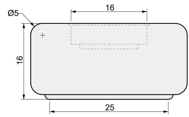
03 SIDE VIEW
