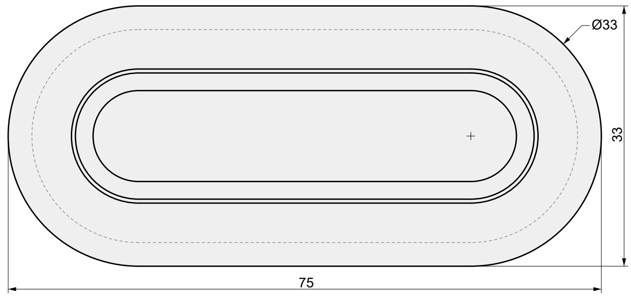
01 TOP VIEW
