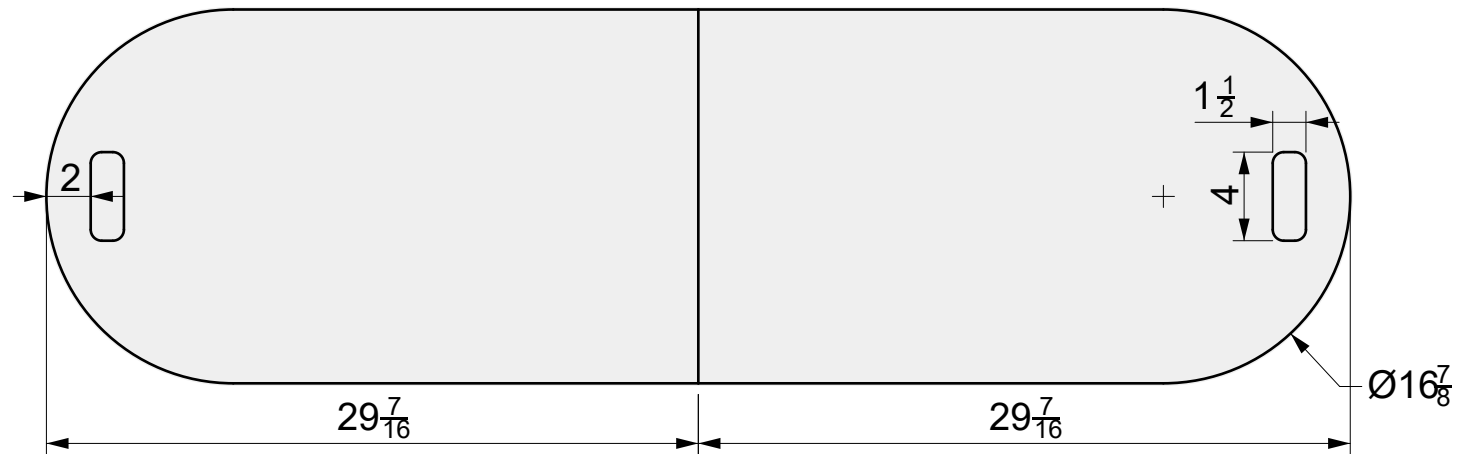
01 TOP VIEW
