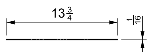
02 FRONT VIEW
