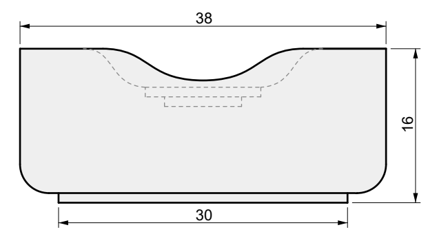
02 FRONT VIEW
