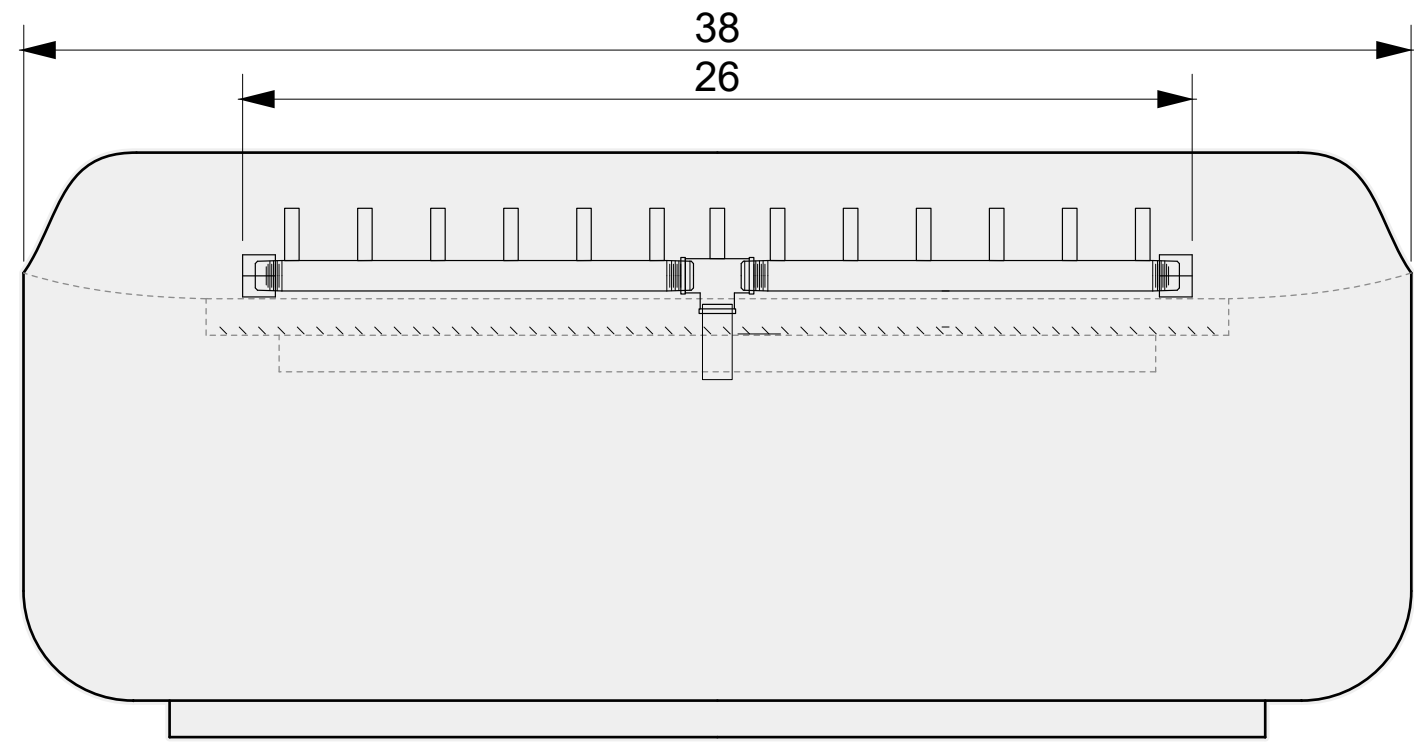
01 SIDE VIEW
