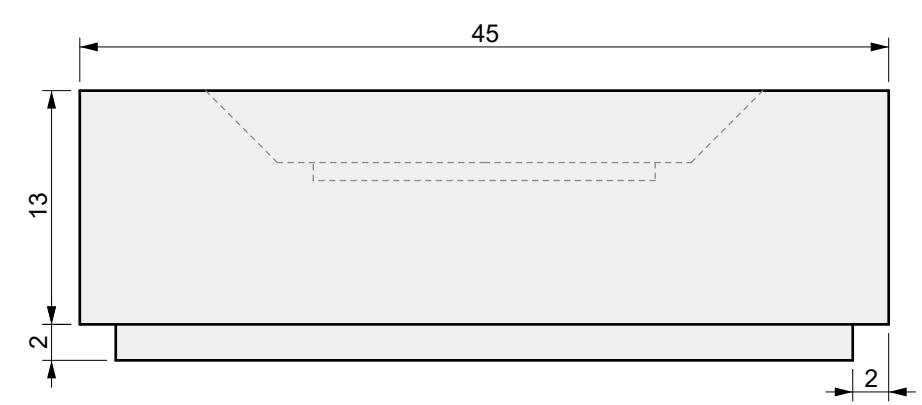
03 SIDE VIEW
