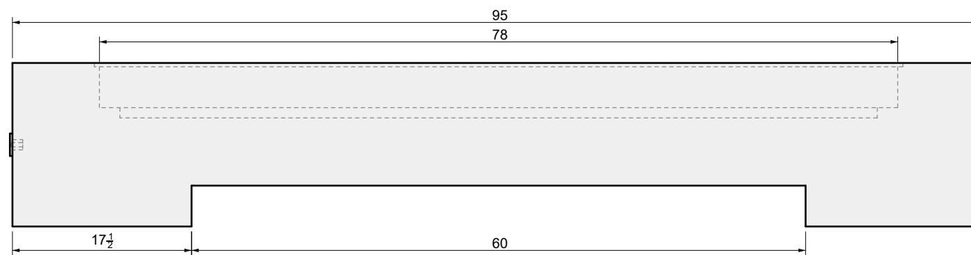
02 FRONT VIEW
