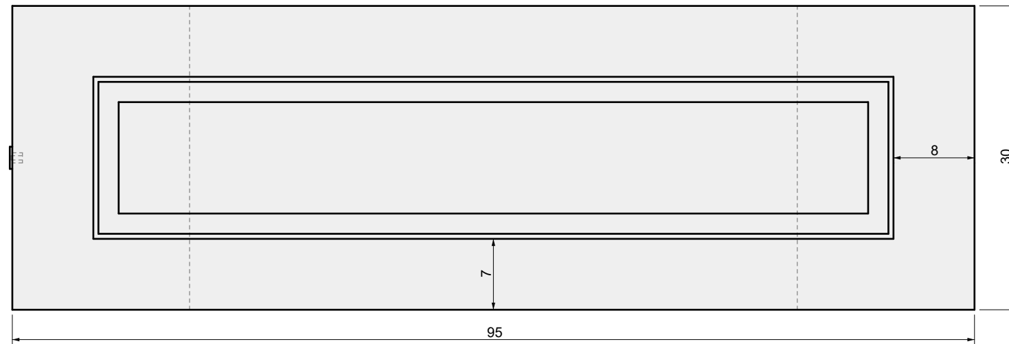
01 TOP VIEW
