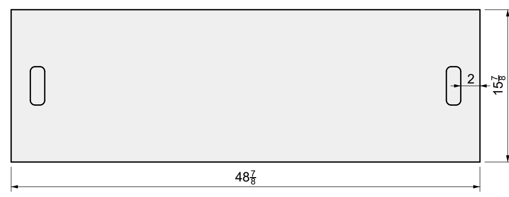
01 TOP VIEW
