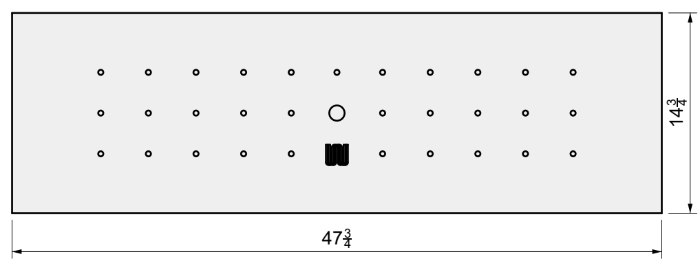
01 TOP VIEW
