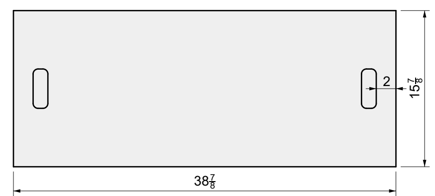
01 TOP VIEW
