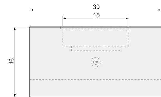
03 SIDE VIEW
