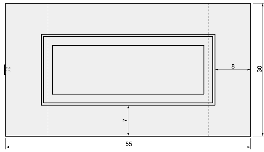
01 TOP VIEW
