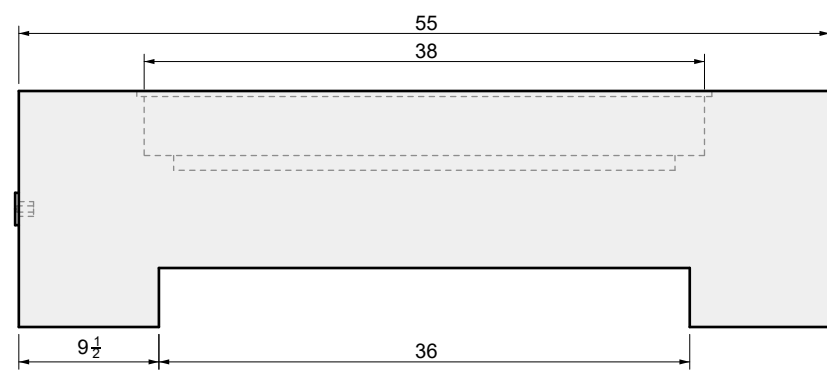
02 FRONT VIEW
