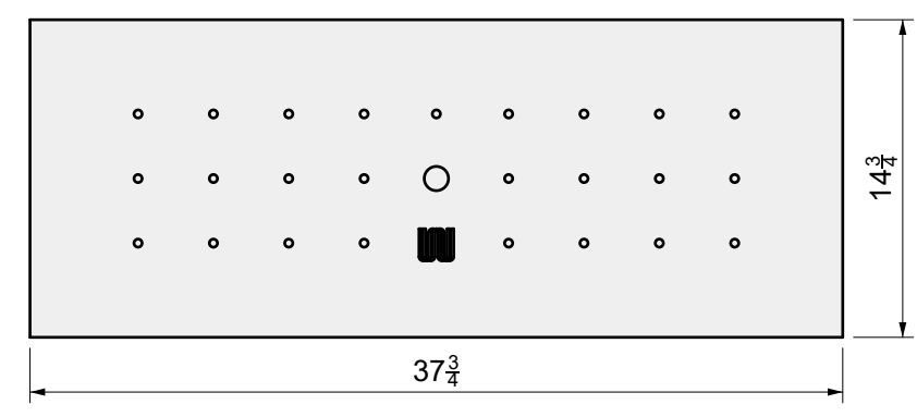
01 TOP VIEW
