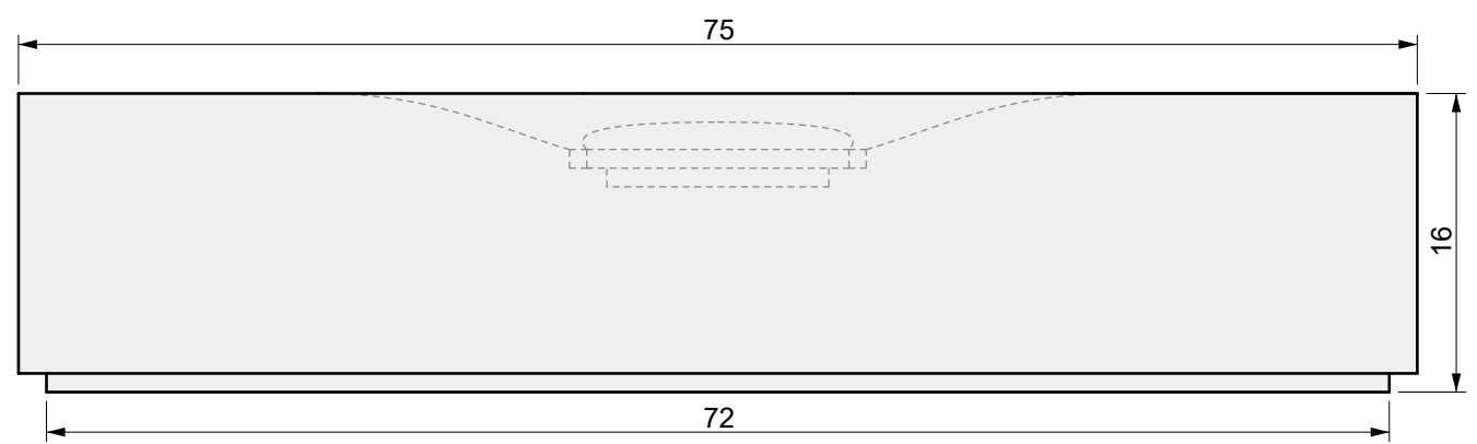
02 FRONT VIEW
