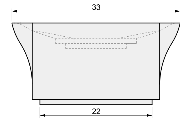
03 SIDE VIEW
