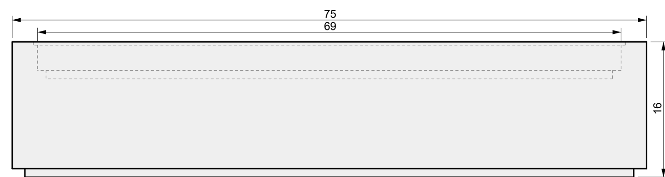
02 FRONT VIEW
