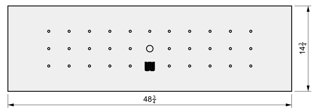
01 TOP VIEW
