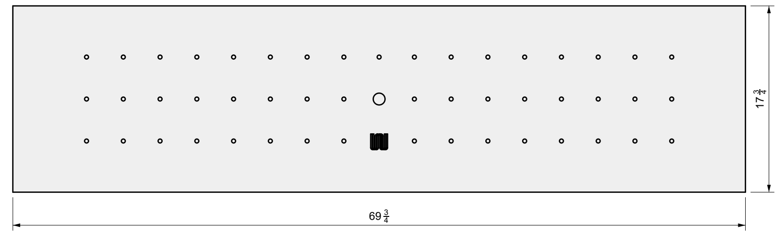
01 TOP VIEW
