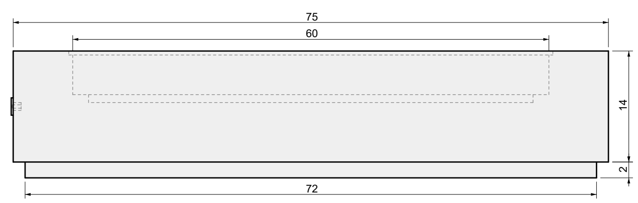
02 FRONT VIEW
