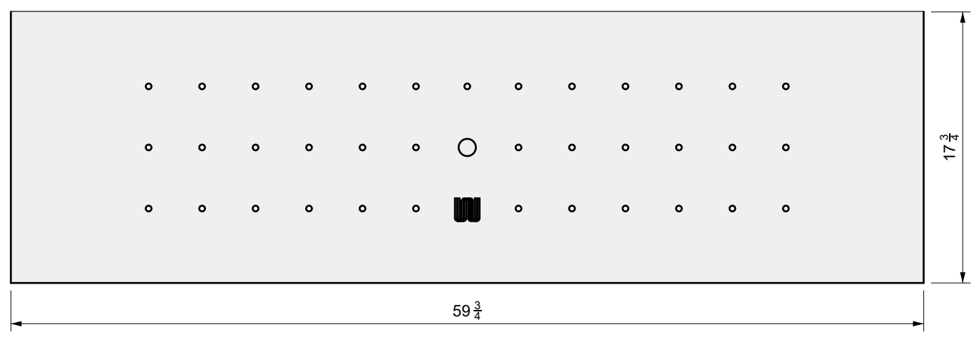
01 TOP VIEW
