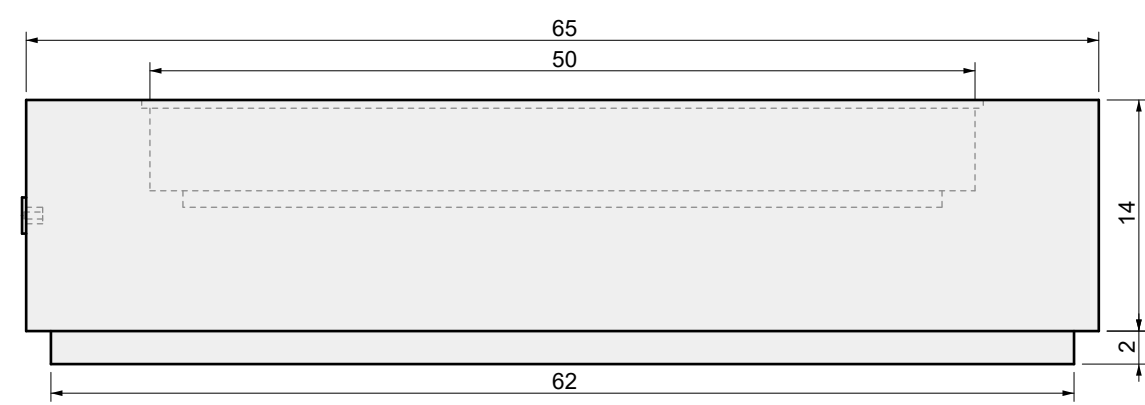
02 FRONT VIEW
