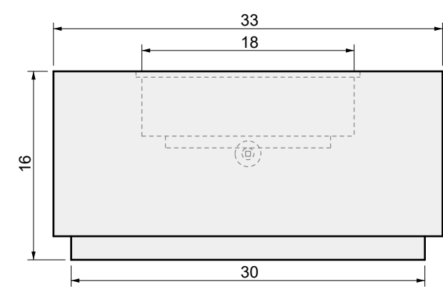
03 SIDE VIEW
