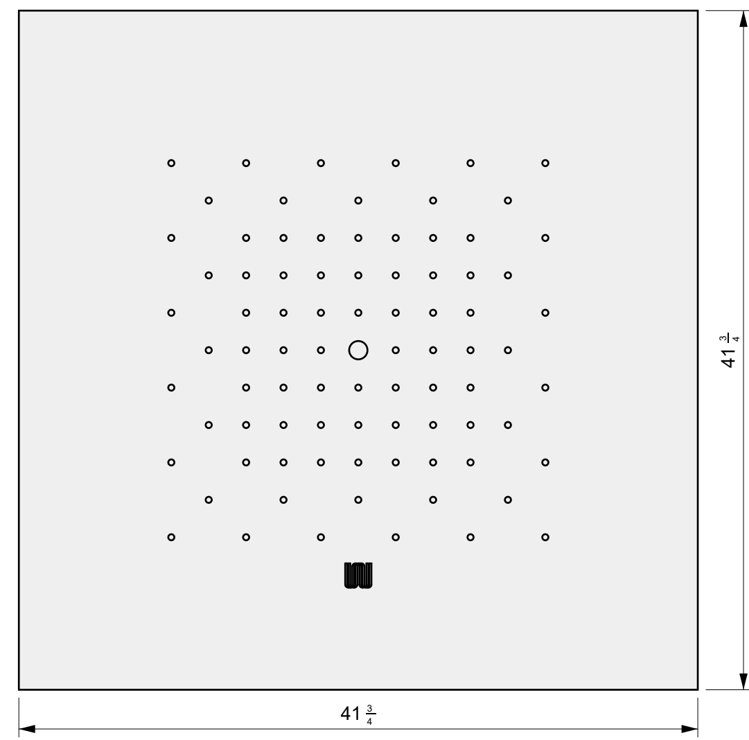
01 TOP VIEW
