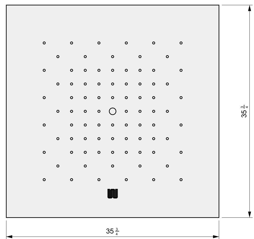
01 TOP VIEW
