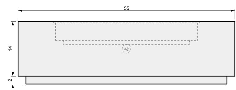
03 SIDE VIEW
