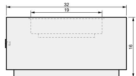
02 FRONT VIEW
