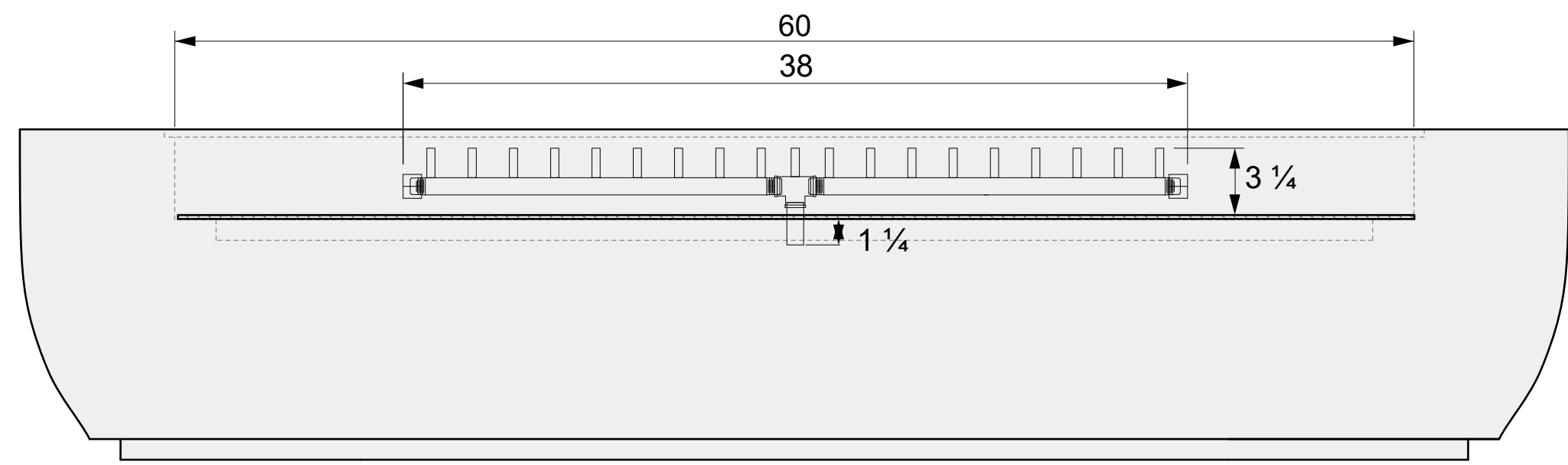
01 SIDE VIEW
