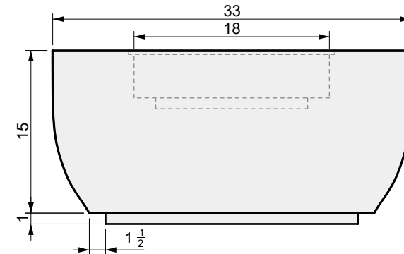
03 SIDE VIEW
