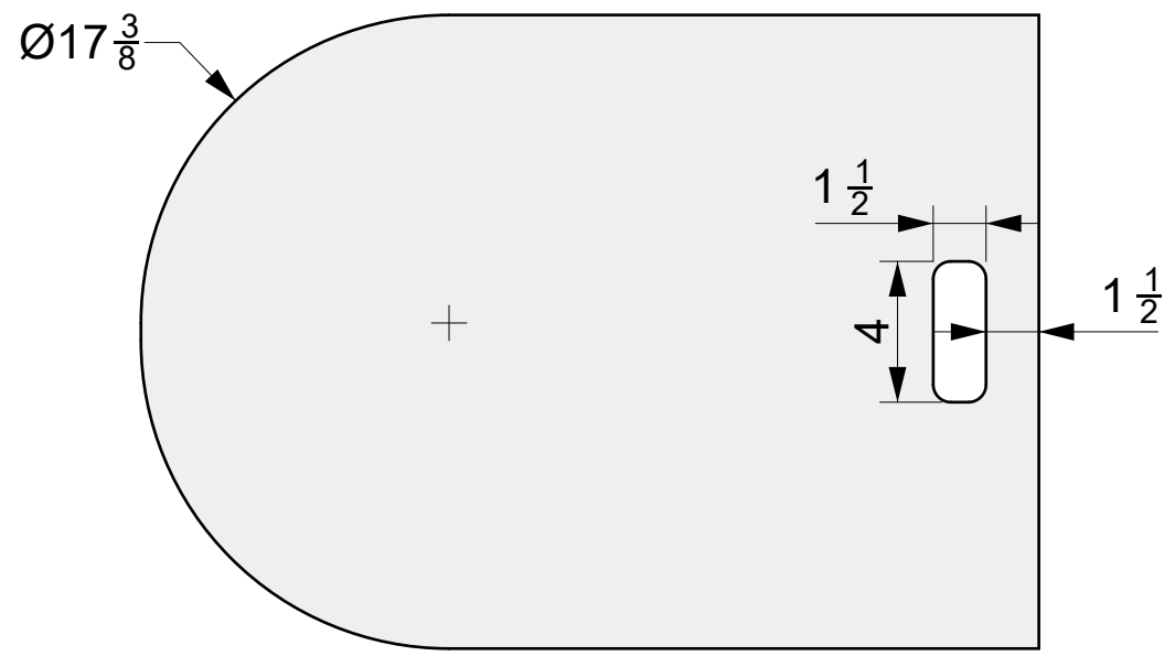
01 TOP VIEW
