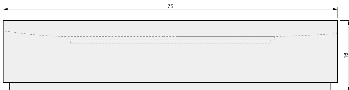
02 FRONT VIEW
