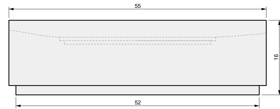
02 FRONT VIEW
