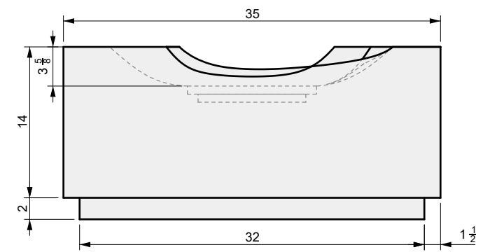
03 SIDE VIEW
