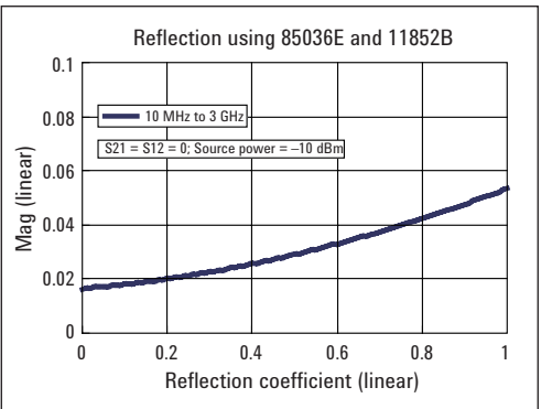
Reflection uncertainty 10 MHz to 3 GHz (typical)
