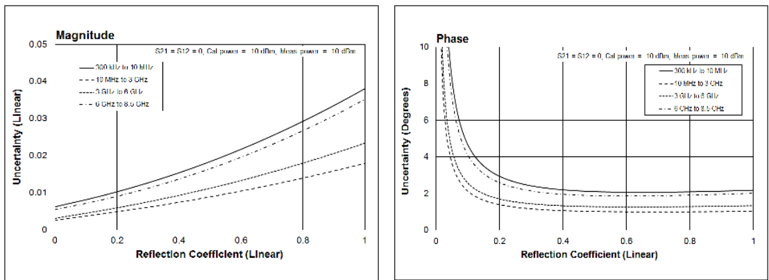
Reflection uncertainty (specification)
