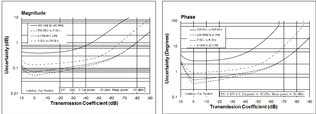
Transmission uncertainty (specification)
