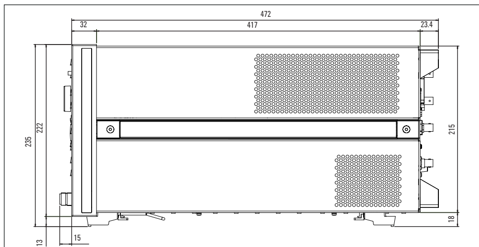
Figure 8. Dimensions (side view, E5071C Option 230/235/240/245/260/265/280/285/430/435/440/445/460/465/480/485, in millimeters)
