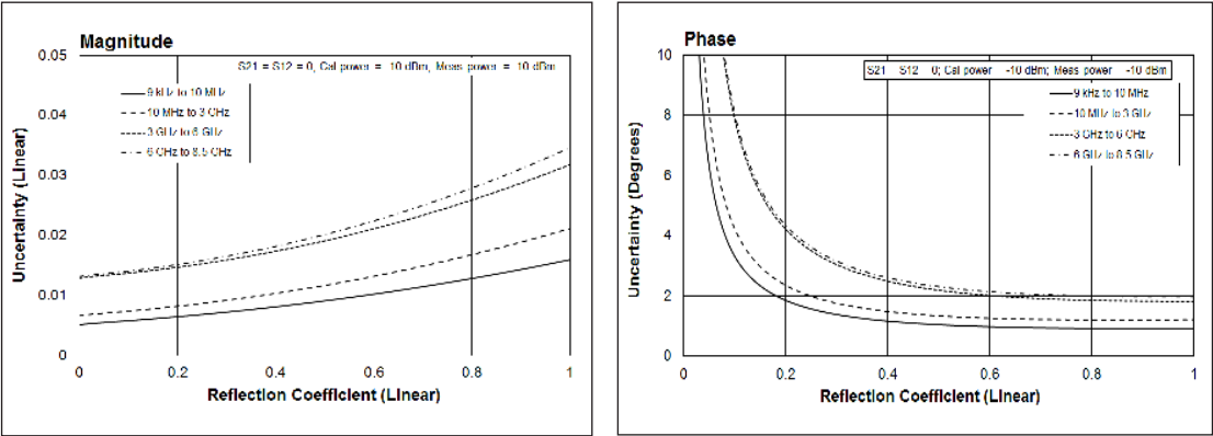
Reflection uncertainty (specification)
