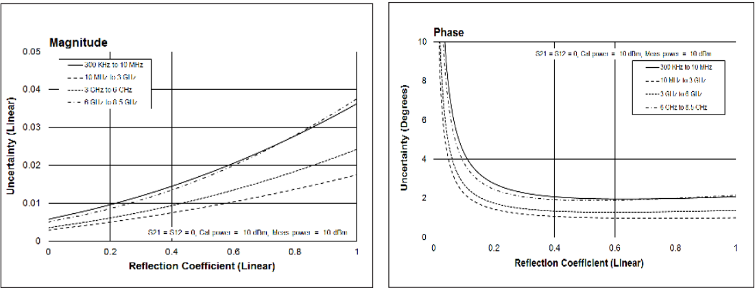
Reflection uncertainty (specification)
