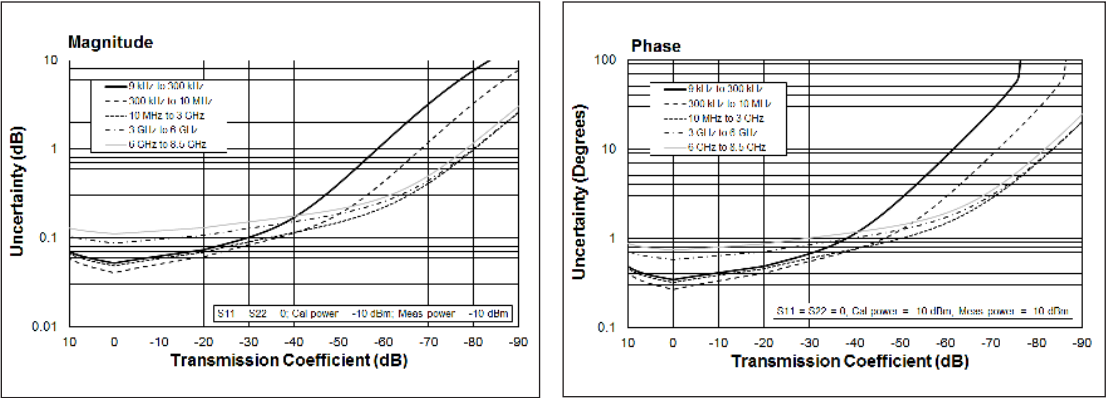
Transmission uncertainty (specification)
