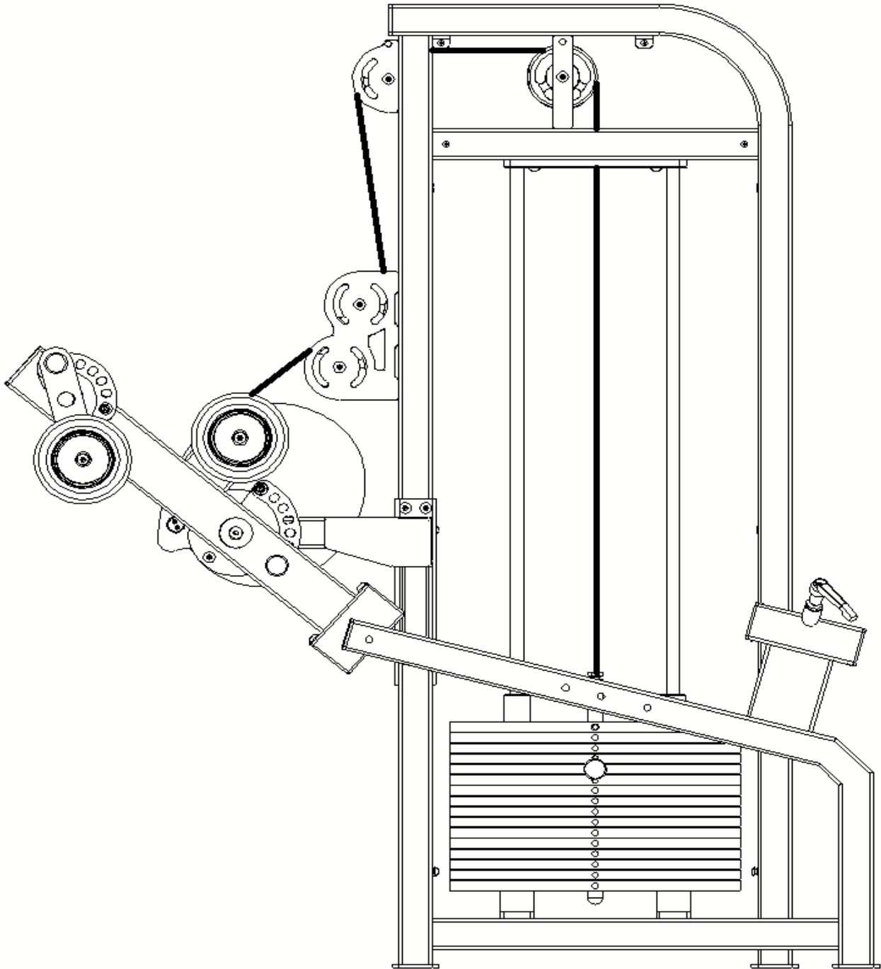
Wire rope routing diagram
