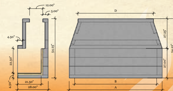
STANDARD LINEAR LAYOUT (NT)
