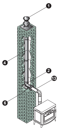
Wood Stove with Stovepipe
