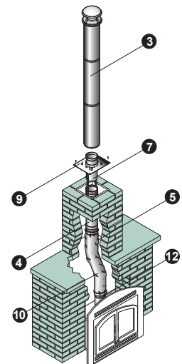
Wood Fireplace Insert
