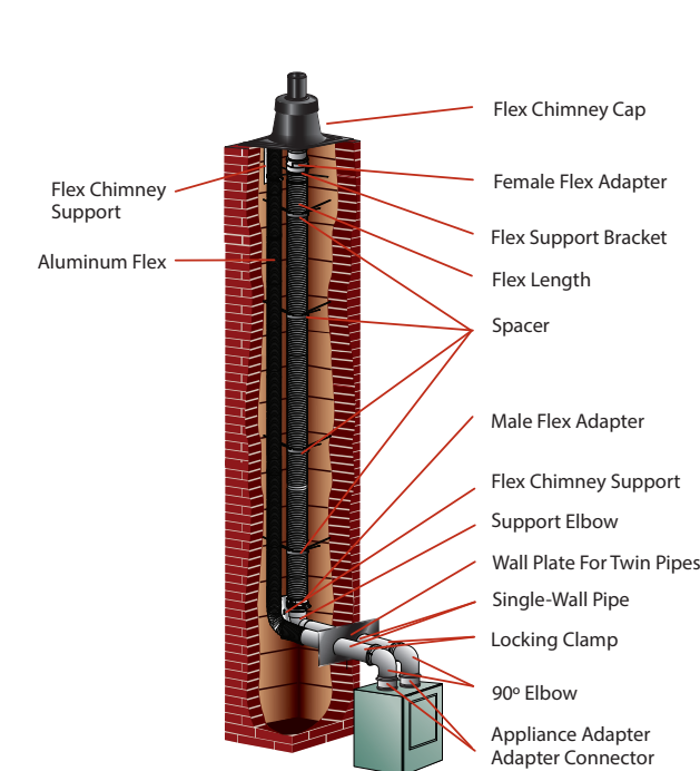
Flex Through Chimney w/ Air Intake
