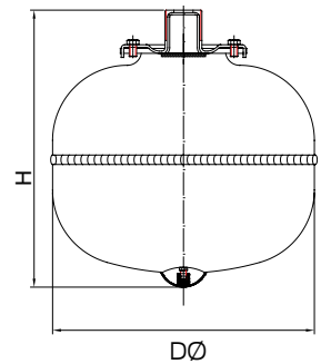
2-35 Ltr models
