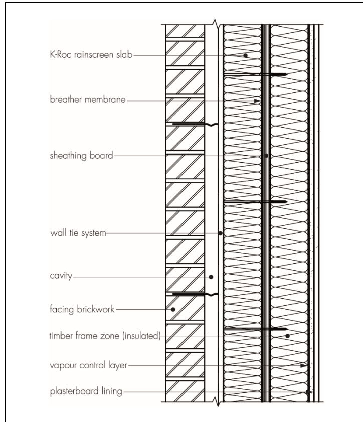
Figure 2 Timber frame application
