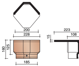
Ventilated angular begin ridge
