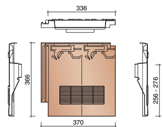
Integrated vent tile
