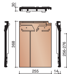
Left tile and a half without interlocking
