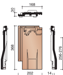
Ventilation tile with synthetic grid
