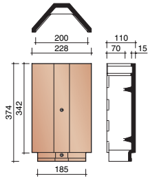
Ventilated angular end hip tile
