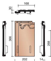
Eave ventilation tile
