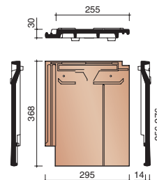
Right tile and a half
