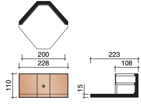
Ventilated angular end ridge
