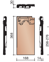
Left tile without side interlocking
