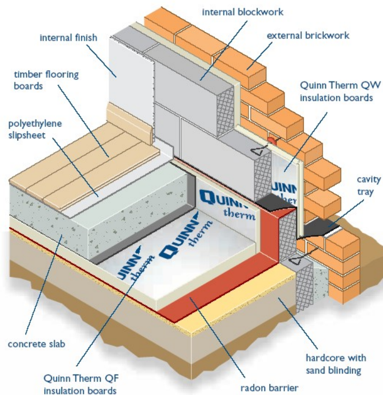
Figure 2: Insulating floors beneath ground bearing concrete slab
