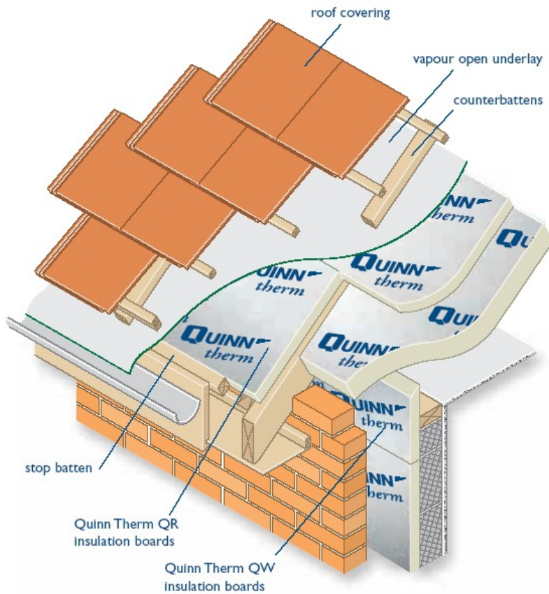
Figure 2: Insulating pitched roofs above and between the rafters
