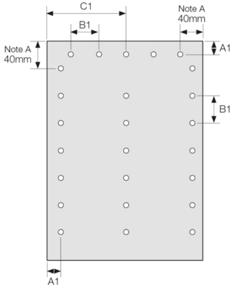
Diagram 1 - typical detail of fixing layout
