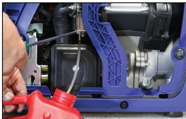
Figure 51 – iGen2200 & 2500 Draining the Carburettor
