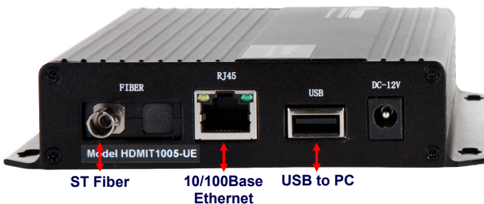
HDMIT1005-UE Rear Panel View
