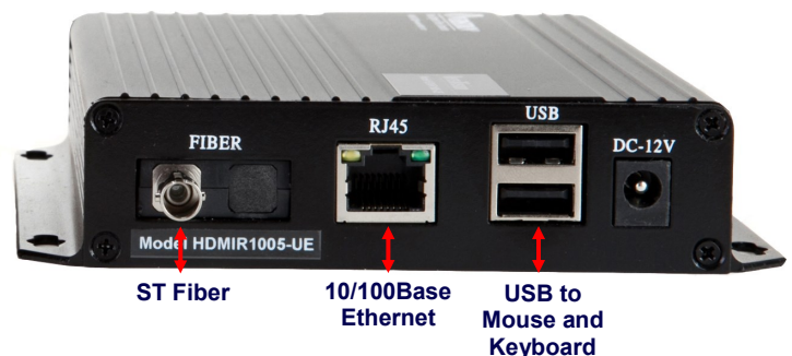
HDMIR1005-UE Rear Panel View
