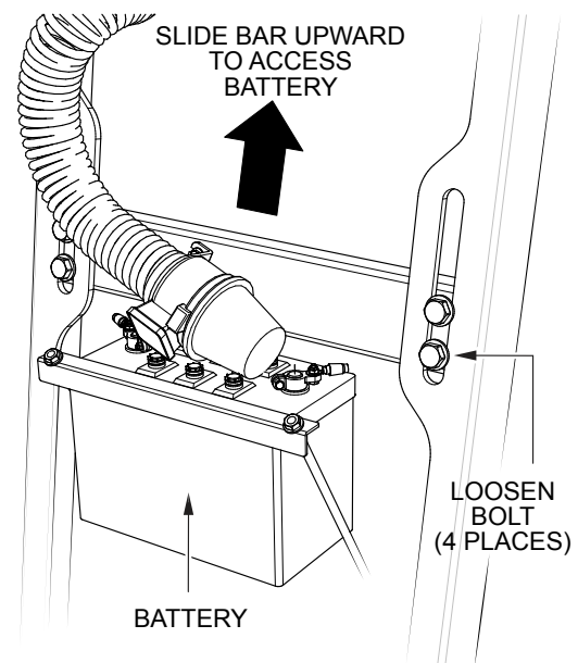
Figure 31. Raising The Battery
