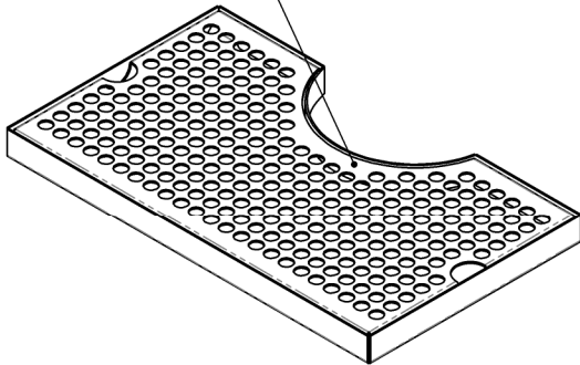
PERFORATED SCREEN (Ø .375 ON .50 CENTERS) STANDARD
